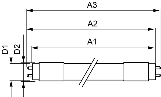
TLED 120V 24-54W 3600lm 3500K G5
